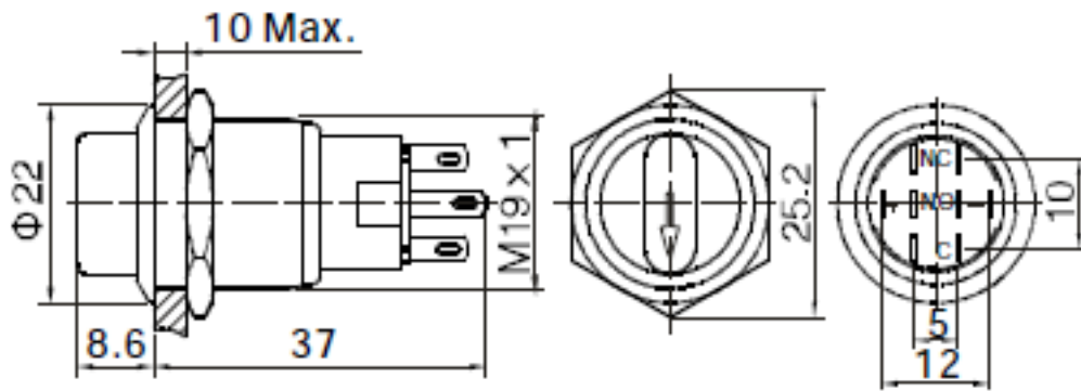
Top View Terminal Arrangement
